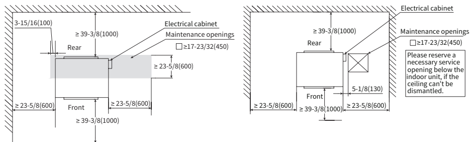
Figure 4.1 Operation and Maintenance Space
